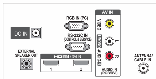
REAR JACK PANEL 26LT560C/22LT560C
